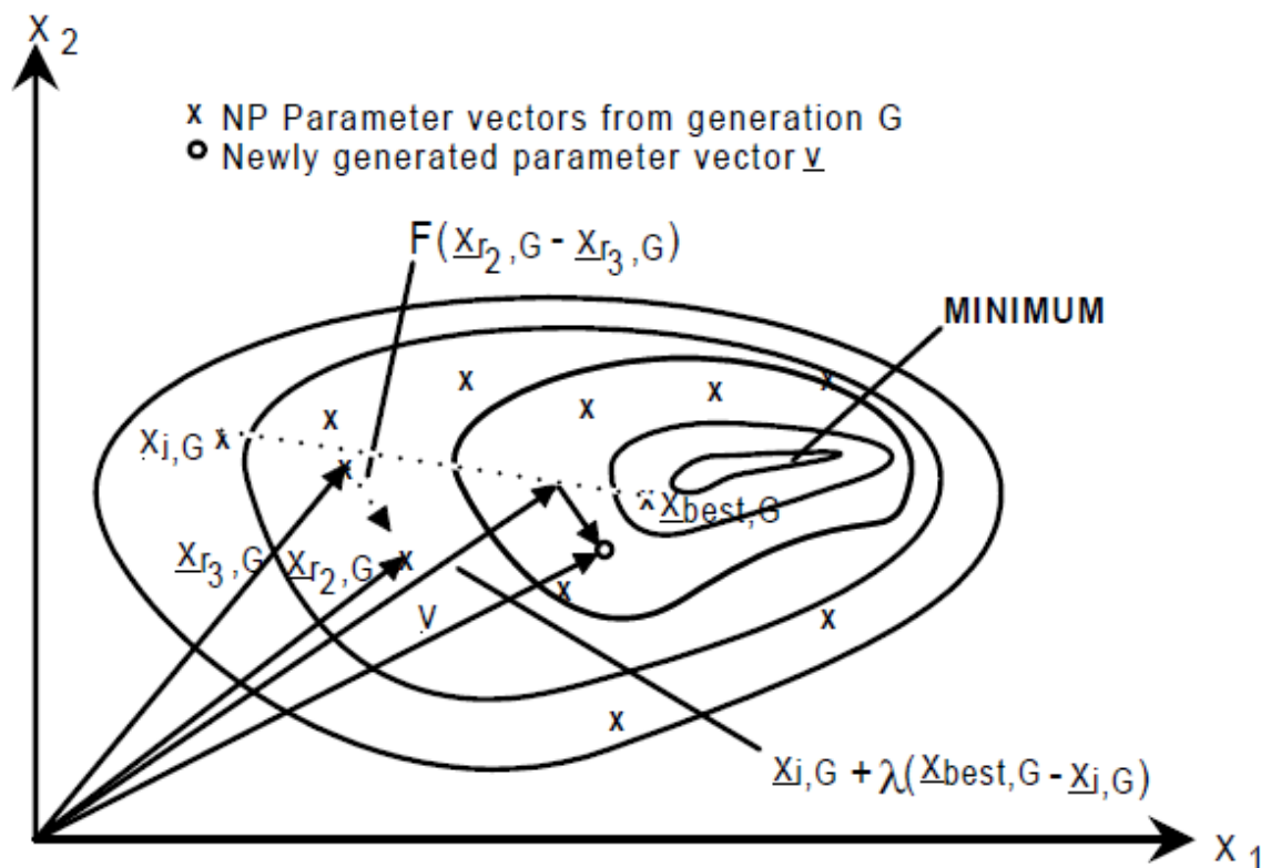
Figure 59: Two dimensional example of an objective function showing its contour lines and the process for generating v in scheme DE2.
